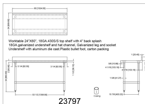
WTG-2460-4BS-418
