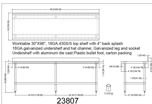
WTG-3096-4BS-418
