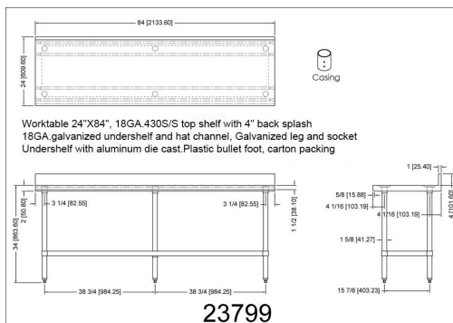
WTG-2484-4BS-418
