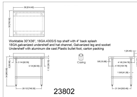
WTG-3036-4BS-418
