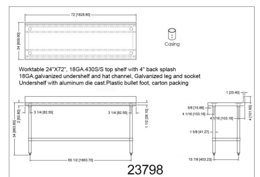
WTG-2472-4BS-418
